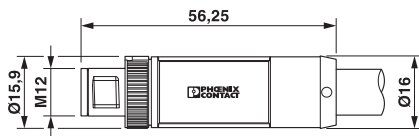
Plug, M12 x 1, straight
